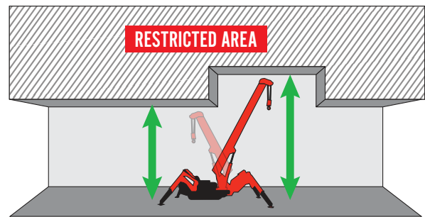
Variable Height Limitation
